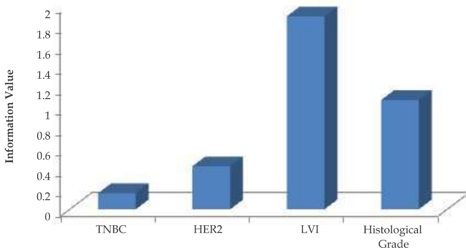
Fig. 2: The bar diagram showing the information value for all the four significant variables with TIL as response variable
